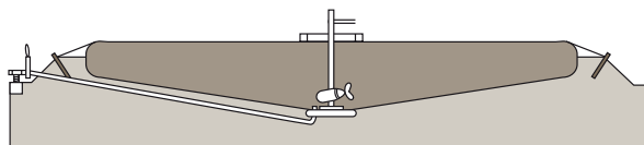
Prierez Alligator Bagtank (plný).
